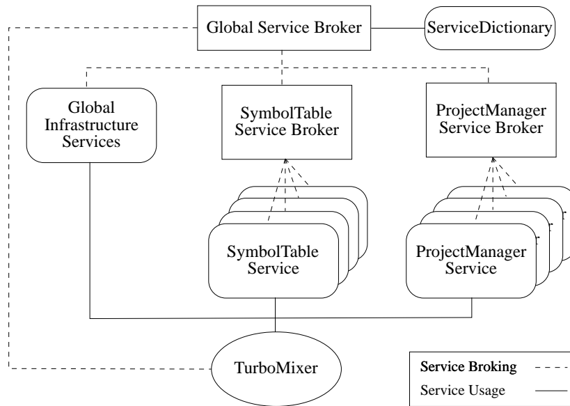
Figure 6. Service broker hierarchy.
