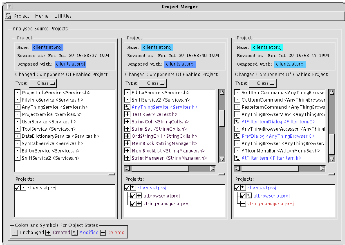
Figure 4. TurboMixer visualizing differences in structure and classes
