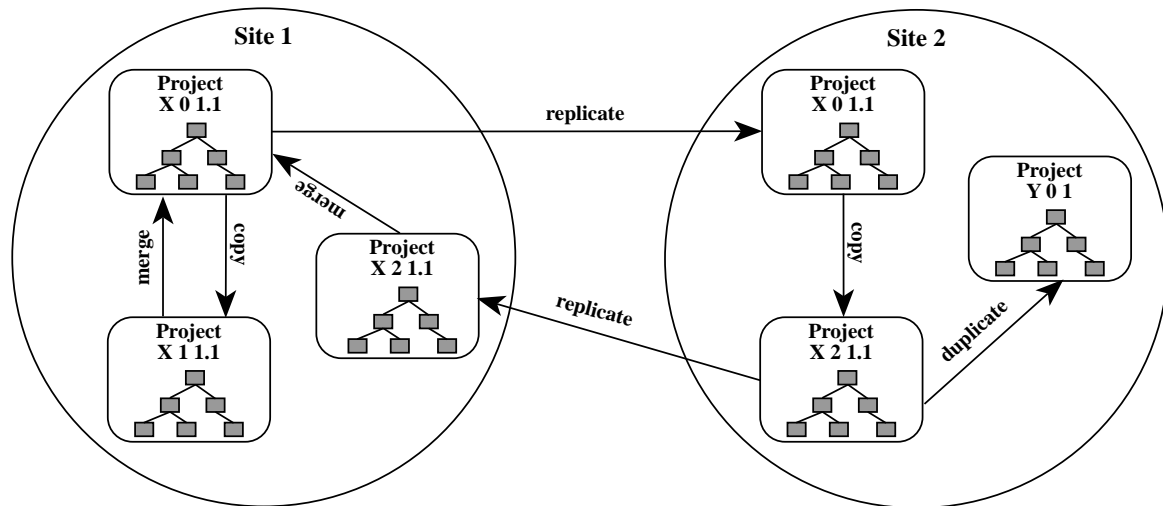
Figure 3. Policy-driven optimistic cooperation with Beyond-Sniff
