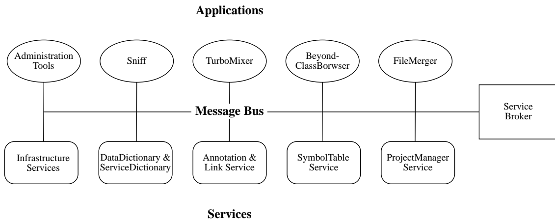
Figure 5. Architecture overview.
