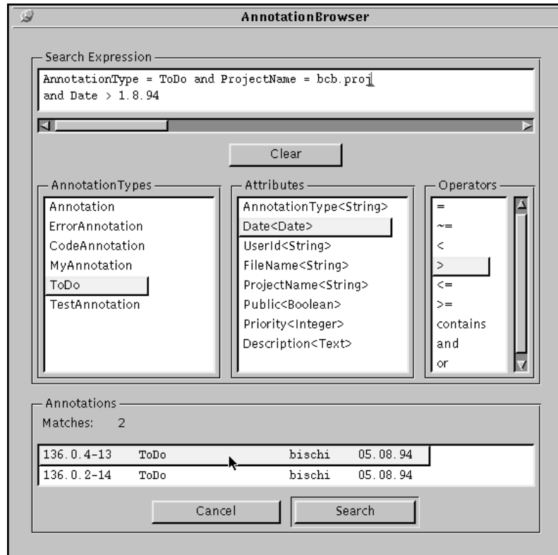
Figure 2. AnnotationBrowser.
